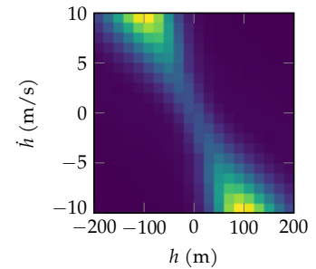
Figure 14.2. Proposal distribution generated from the probability of collision when following the optimal collision avoidance policies from different initial states with t_{\text{col}} = 20\text{s} and a_{\text{prev}} = 0\text{m/s} . Yellow indicates higher probability density.
