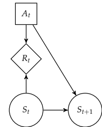
Figure 7.2. Stationary MDP decision network diagram. All MDPs have this general structure.
